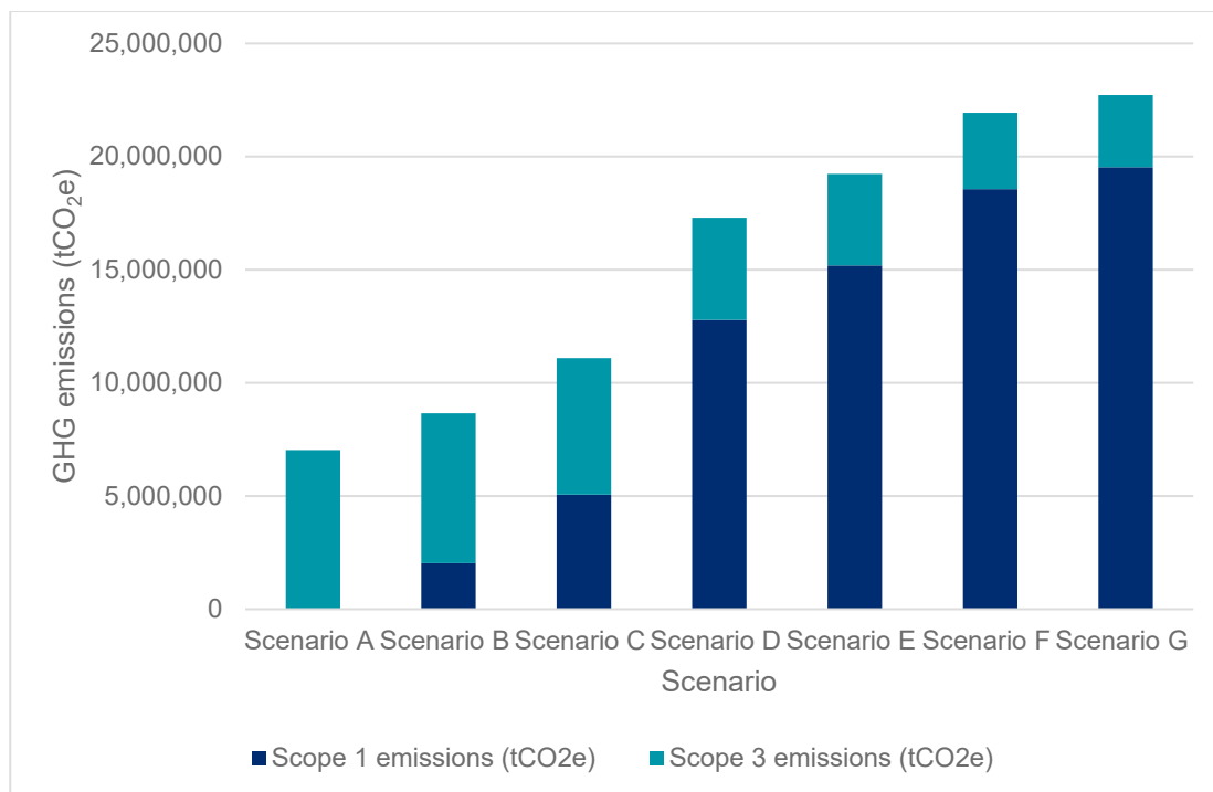
Plate 5: B6 Operational GHG Emissions of the Modelled Operating Scenarios for the Proposed Development Broken Down by Emissions Source
